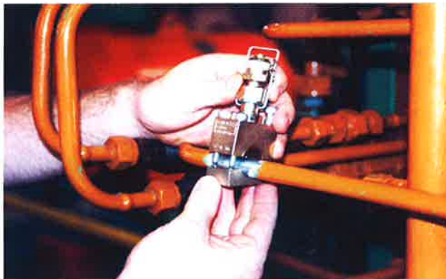
Installation on non-pressurized pipe serv-Clip ® 2
